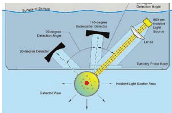
Figure 4. An In-Situ probe turbidimeter with a ratio design. The In-situ designates the measurement to be made in the process (the river, lake, sample transport pipe) itself. Two detectors extend the range of measurement to low turbidity levels and reduce color interference.
