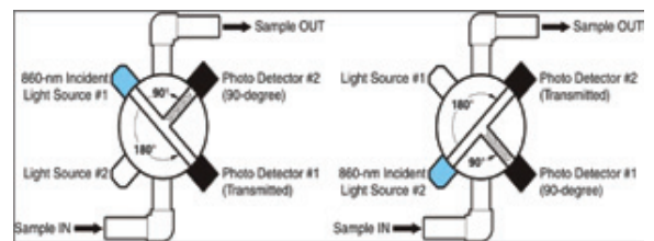
Figure 5. A dual-light source, dual-detector design. Two LED light two detectors combine to perform the turbidity measurement. The measurement consists of two phases.
