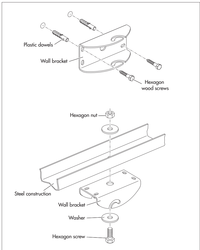
Fig. 7: Fasten the wall bracket of the swivel mount. Fastening of the housing bracket is carried out in the same way.
