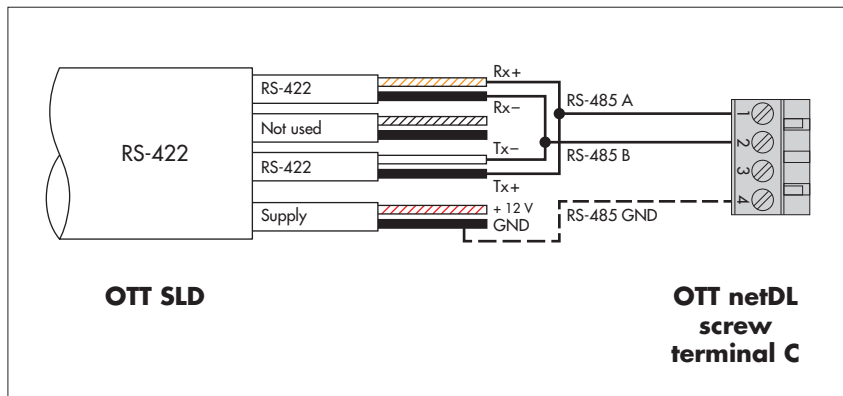
Fig. 31: Connecting the OTT SLD to the OTT netDL using the RS-485 interface (SDI-12 via RS-485).
