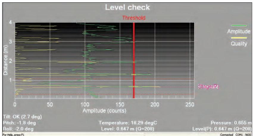
Fig. 19: "Level check" evaluation window.
