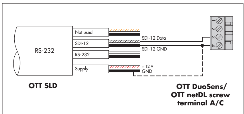
Fig. 29: Connecting the OTT SLD to OTT DuoSens/OTT netDL using the SDI-12 interface.
