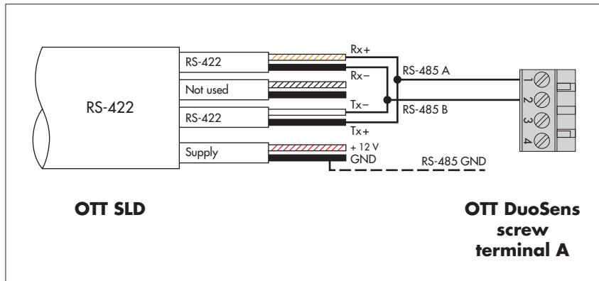
Fig. 30: Connecting the OTT SLD to the OTT DuoSens using the RS-485 interface (SDI-12 via RS-485).
