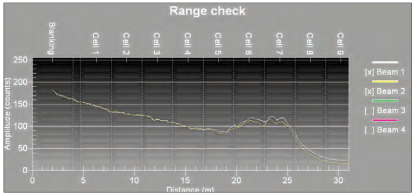
Fig. 22: Successful range check.
