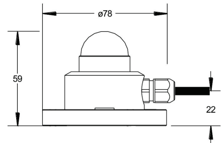
Dimensions of LP02 Sensor in mm
